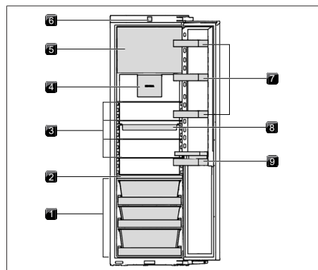
Fig. 5.2 Composition C178KGF
