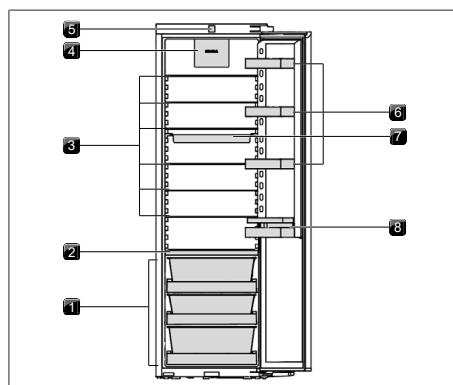
Fig. 5.1 Composition C178K
