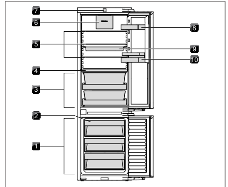
Fig. 5.4 Composition C178KGW
